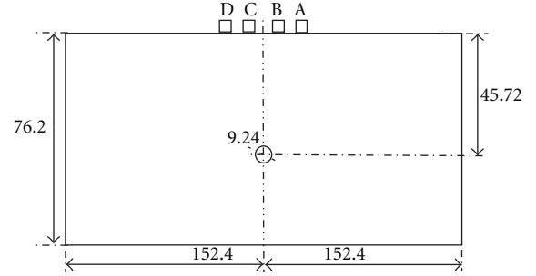
FIGURE 7: Dimensions of the aluminum alloy (unit: mm).
